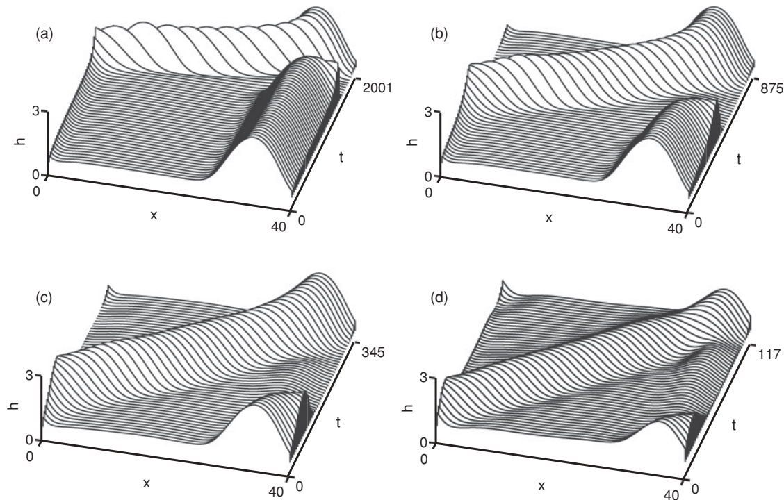
FIG. 8. Space-time plots of the time evolution of stick-slip ridge (SSR) solutions beyond depinning via a Hopf bifurcation over one period in space and time at (a) \mu = 0.011414 close to the saddle node of the SSR branch at \mu_{\text{sn4}}^{2d} = 0.01141303 with temporal period T = 2000.6 , (b) \mu = 0.012 with T = 875.0 , (c) \mu = 0.02 with T = 345.0 , and (d) far from depinning, \mu = 0.06 with T = 116.8 .
