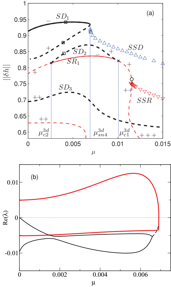
FIG. 23. (Color online) Scenario (iii): Bifurcation diagram for steady ridges (SR, thin red lines), and steady drops (SD, black lines) on a substrate with hydrophobic line defects (wettability contrast \epsilon = 0.3 ) and spanwise system size L = 29 showing the L^2 norm \|\delta h\| of steady solutions as a function of the driving force \mu . Solid (dashed) lines denote stable (unstable) solutions. Downward (upward) pointing triangles indicate SSR (SSD) solutions. Solution profiles at locations indicated by open squares are shown in Fig. 24. The remaining parameters are as in Fig. 3. The SD_3 branch becomes stable at \mu = 0.062 (off scale). (b) Real part of the leading eigenvalues for the stable (thin black line) and unstable part (heavy red line) of SD_1 drop branch. The black dashed line corresponds to a complex eigenvalue.
