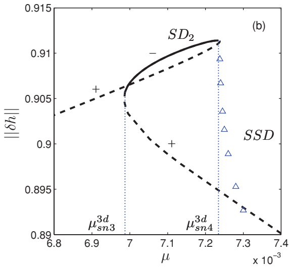
FIG. 21. (Color online) Scenario (iib): (a) Bifurcation diagram for steady ridges (SR, thin red lines), and steady drops (SD, black lines) pinned by a hydrophobic line defect of strength \epsilon = 0.3 for L = 27.8 showing the L^2 norm \|\delta h\| of steady solutions as a function of the driving force \mu . Solid (dashed) lines denote stable (unstable) solutions. (b) shows a zoom of the cusplike feature on the SD_2 branch. The SD_3 branch becomes stable at \mu = 0.064 (not shown). Downward (upward) pointing triangles indicate SSR (SSD) solutions. Solution profiles at locations indicated by open squares are shown in Fig. 22. The remaining parameters are the same as in Fig. 3.
