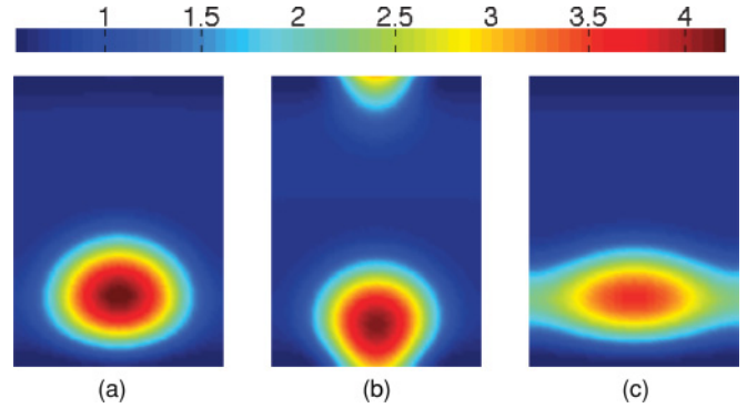
FIG. 24. (Color online) Scenario (iii): Steady states at locations indicated by open squares in Fig. 23 in terms of contours of constant h(x, y) , ordered by decreasing norm. (a) \mu = 0.00419 , (b) \mu = 0.00391 , and (c) \mu = 0.00401 . The remaining parameters are as in Fig. 3.
