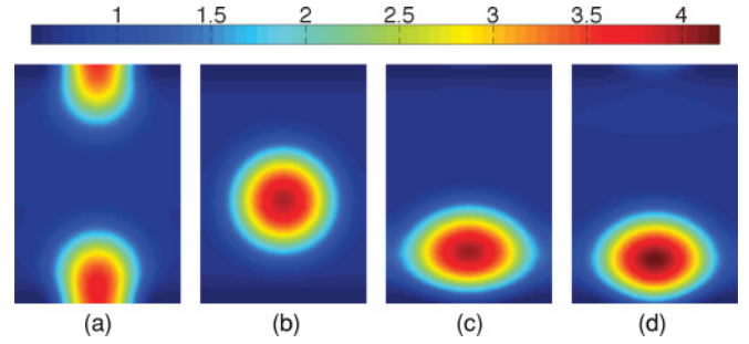
FIG. 22. (Color online) Scenario (iib): Steady states at locations indicated by open squares in Fig. 21 in terms of contours of constant h(x, y) . (a) \mu = 0.00082 on the unstable part of the drop branch SD_1 , (b) on the stable part of the drop branch SD_1 at \mu = 0.00110 , (c) at the saddle-node \mu_{sn2}^{3d} = 0.00582 on SD_1 , and (d) at the sniper bifurcation at \mu_{sn4}^{3d} = 0.00724 on SD_2 .
