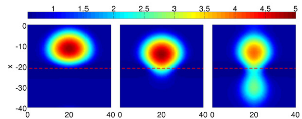
Fig. 6: (Colour on-line) Shown are contours of steady-drop solutions for a hydrophobic defect for \mu = 4 \cdot 10^{-3} . From left to right, profiles correspond to crosses in fig. 5 from large to small norm. That is, the left panel shows the stable pinned drop. The thin line marks the minimum of wettability.
