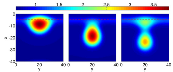
Fig. 3: (Colour on-line) Shown are contours of steady-drop solutions for a hydrophilic defect for \mu = 3.5 \cdot 10^{-3} . From left to right, profiles correspond to crosses in fig. 2 from large to small norm, i.e. , the left panel shows the stable pinned drop. The thin line marks the maximum of wettability.
