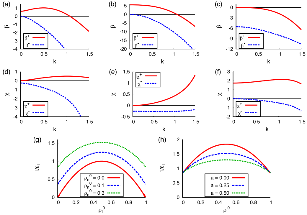
Figure 5. (a)–(f) Dispersion relations for the case when \epsilon_n \epsilon_1 > \epsilon_{nl}^2 , \epsilon_n f_{nl} + \epsilon_l f_{nn} - 2\epsilon_{nl} f_{nl} > 0 (i.e. in equation (51) a > 0 , b > 0 ) and k_B T = 1 . The graphs in the top row show \beta(k) and the graphs in the middle row show \chi(k) . In (a) and (d) the parameters are: \rho_1^0 = 0.648 , \rho_n^0 = 0.3 , \epsilon_1 = 1.25 , \epsilon_n = 0.5 , \epsilon_{nl} = 0.6 , \mu = -3.35 , M^n = 1 , M_c^l = 0 and M_{nc}^l = 1 . In (b) and (e) the parameters are: \rho_1^0 = 0.648 , \rho_n^0 = 0.3 , \epsilon_1 = 1.25 , \epsilon_n = 0.5 , \epsilon_{nl} = 0.6 , \mu = -3.35 , M^n = 1 , M_c^l = 0 and M_{nc}^l = 9 . In (c) and (f) the parameters are: \rho_1^0 = 0.901 , \rho_n^0 = 0.3 , \epsilon_1 = 1.4 , \epsilon_n = 0.6 , \epsilon_{nl} = 0.8 , \mu = -3.8 , M^n = 1 , M_c^l = 0 and M_{nc}^l = 1 . (g) shows how the spinodal line shifts for increasing \rho_n^0 , where \epsilon_n \epsilon_1 - \epsilon_{nl}^2 = 0.25 , \epsilon_n = \epsilon_1 and k_B T = 1 . (h) shows how the spinodal line shifts as the value of a = \epsilon_n \epsilon_1 - \epsilon_{nl}^2 increases, when \rho_n^0 = 0.3 , \epsilon_n = \epsilon_1 and k_B T = 1 .
