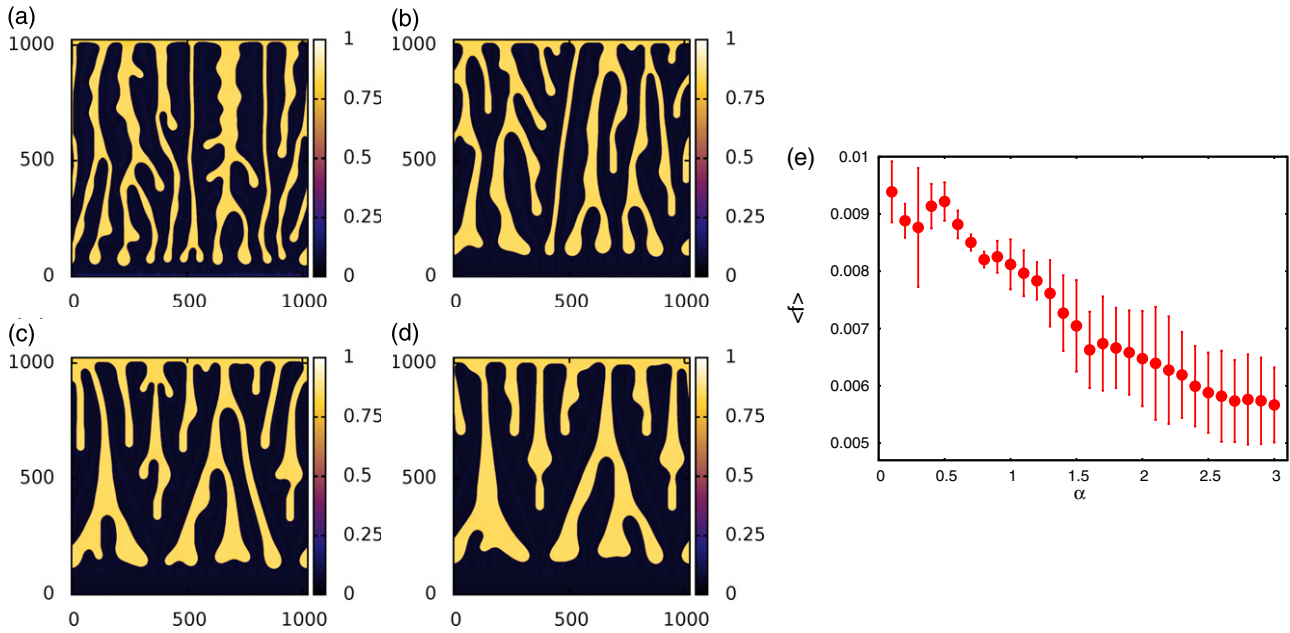
Figure 10. Nanoparticle density profiles for calculations with (a) \alpha = 0.1 , (b) \alpha = 1 , (c) \alpha = 2 and (d) \alpha = 3 . In (e) we display a plot showing the dependence of the number of fingers on the parameter value \alpha . The parameter values are: k_B T = 1 , \epsilon_1 = 1.4 , \epsilon_n = 0.6 , \epsilon_{nl} = 0.8 , M_1^c = 0 , M_1^{nc} = 1 , \beta\mu = -3.8 , \Delta x = 1 and \lambda = 0.1 .
