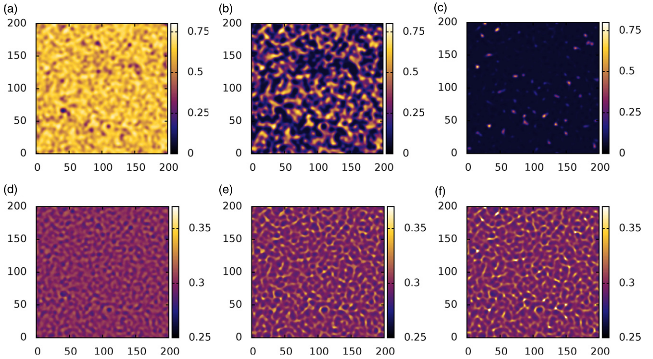
Figure 6. Density profiles displaying evaporation via spinodal decomposition. The top row shows the liquid density profiles and the bottom row shows the nanoparticle profiles at times t/t_1 = 7 (left), t/t_1 = 8 (centre) and t/t_1 = 9 (right), where t_1 \equiv \frac{\beta}{M_1^{nc}} . The system parameter values are: k_B T = 1 , \epsilon_1 = 1.4 , \epsilon_n = 0.6 , \epsilon_{nl} = 0.8 , M_1^c = 0 , M_1^{nc} = 1 , \alpha = 0.5 , \beta\mu = -4.08 and \lambda = 0.005 .
