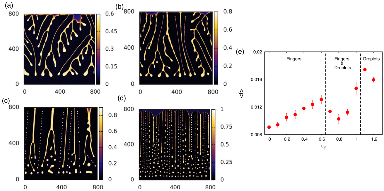
Figure 12. Nanoparticle density profiles for (a) \epsilon_n = 0.3 , (b) \epsilon_n = 0.6 , (c) \epsilon_n = 0.8 and (d) \epsilon_n = 1.1 . In (e) we display a plot showing how the mean number of fingers ( f ) depends on the parameter \epsilon_n . When \epsilon_n > 0.6 we begin to observe droplets being deposited along with the branched structures (as shown in (c)). The parameter values for these calculations are: k_B T = 1 , \epsilon_1 = 1.7 , \epsilon_{n1} = 1.0 , M_1^c = 0 , M_1^{nc} = 1 , \alpha = 0.5 , \mu = -4 , \rho_n^{av} = 0.1 and \lambda = 0.025 .
