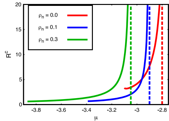
Figure 8. The solid lines display the critical hole radius R^c in units of the lattice grid spacing \sigma versus the chemical potential \mu for different nanoparticle densities \rho_n . The lines start at the lowest value of \mu for which the system is linearly stable. The dotted lines show the value of the chemical potential at coexistence \mu_{\text{coex}} , which the curves approach asymptotically. Here k_B T = 1 , \epsilon_1 = 1.4 , \epsilon_n = 0.6 and \epsilon_{nl} = 0.8 .
