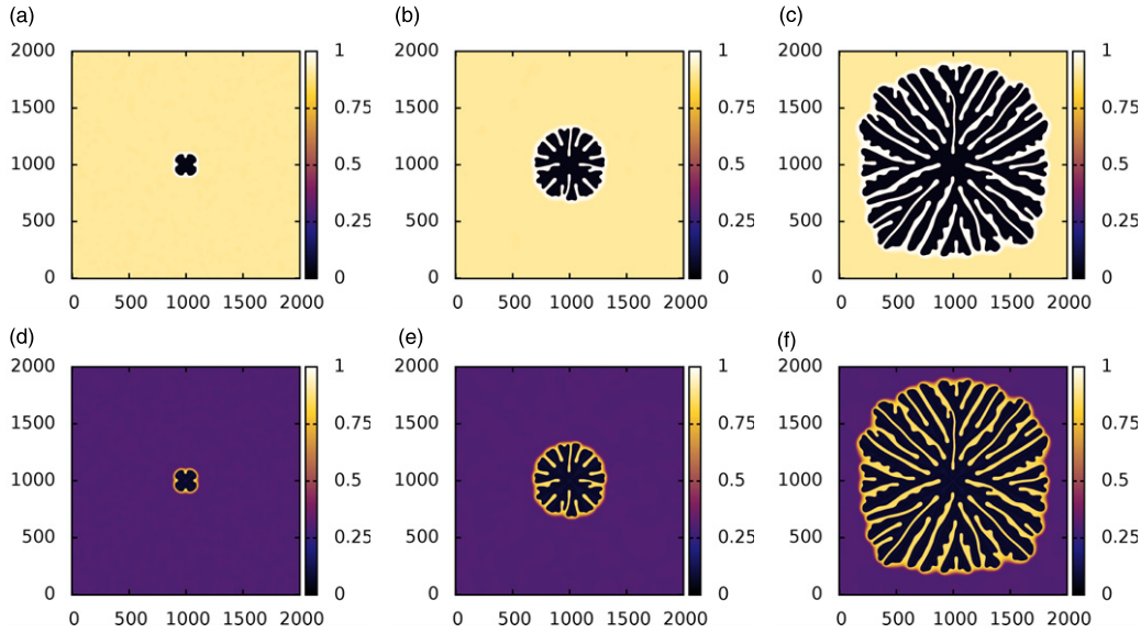
Figure 9. Density profiles displaying the growth of an artificially nucleated hole which develops branched structures. The top row shows the liquid density profiles and the bottom row shows the nanoparticle profiles at times t/t_1 = 2000 (left), t/t_1 = 10\,000 (centre) and t/t_1 = 30\,000 (right). The system parameter values are: k_B T = 1 , \epsilon_1 = 1.4 , \epsilon_n = 0.6 , \epsilon_{nl} = 0.8 , M_1^c = 0 , M_1^{nc} = 1 , \alpha = 0.5 , \beta\mu = -3.8 and \lambda = 0.1 . Note that instead of using equation (53), here the Laplacian term is approximated using: \nabla^2 \rho = \frac{1}{6(\Delta x)^2} (\sum 4\rho^{NN} + \sum \rho^{NNN} - 20\rho) .
