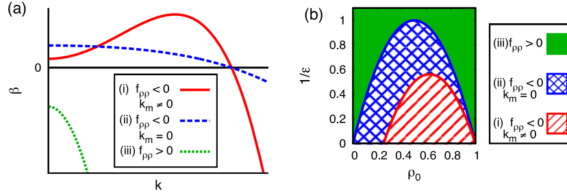
Figure 3. There are three possible forms for \beta(k) : (a) shows an example of each form and (b) shows the regions in parameter space where these different types of \beta(k) curves occur, for the case when M_{nc}/M_c = 1 and k_B T = 1 .
