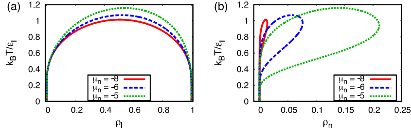
Figure 4. Binodal curves for the binary mixture for varying fixed values of the chemical potential of the nanoparticles \mu_n , for the case when \epsilon_n/\epsilon_l = 0.43 and \epsilon_{nl}/\epsilon_l = 0.57 .
