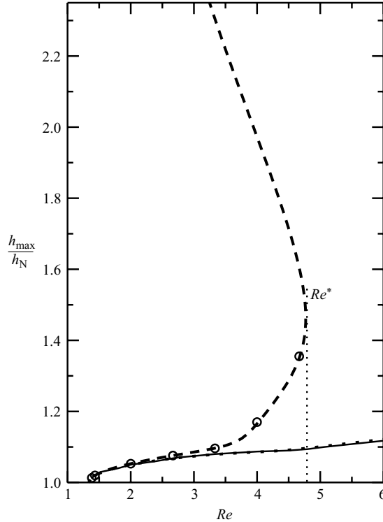
FIGURE 2. Maximum thickness of travelling-wave solutions h_{\max}/h_{\text{N}} as a function of Re , computed with the BE (dashed curve) and the WIBL model (dot-dashed curve) under the closed flow condition for a film falling on a vertical ( S=1 ) and isothermal ( Ma=0 ) wall; We=1000 and \varepsilon_L=0.04/2\pi . For comparison, results of the Navier–Stokes equations (solid curve) obtained by Salamon et al. (1994) as well as results from time-dependent simulations of the BE (circles) obtained by Oron & Gottlieb (2002) are displayed.
